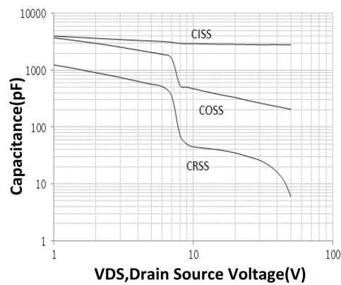
Capacitance Characteristics
