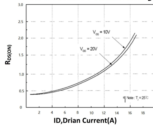
On-Resistance Variation vs. I_D
