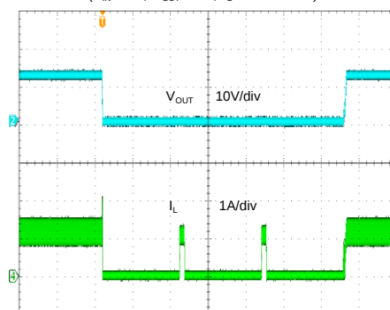
Hard Short Protection ( V_{IN}=48V , V_{OUT}=12V , I_O=1.2A \sim Short)
