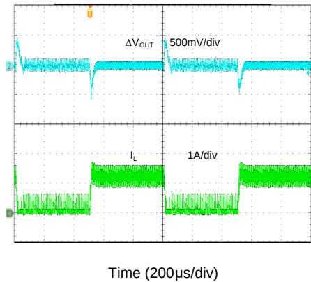
Load Transient ( V_{\text{IN}}=48\text{V}, V_{\text{OUT}}=12\text{V}, I_{\text{O}}=0.12 \sim 1.2\text{A} )
