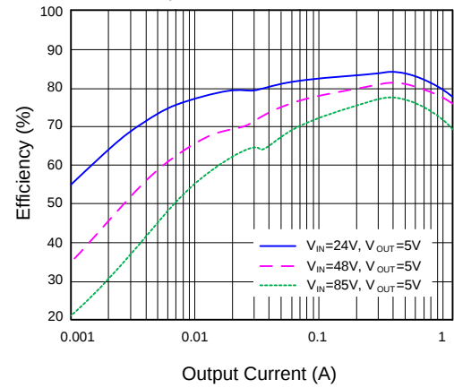
Efficiency vs. Output Current ( L=47\mu\text{H}/\text{CDRH8D43-470NC} )
