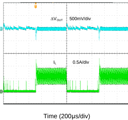
Load Transient ( V_{\text{IN}}=48\text{V}, V_{\text{OUT}}=12\text{V}, I_{\text{O}}=0 \sim 0.6\text{A} )
