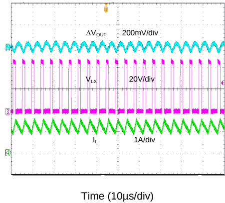
Output Ripple ( V_{\text{IN}}=48\text{V}, V_{\text{OUT}}=12\text{V}, I_{\text{O}}=1.2\text{A} )
