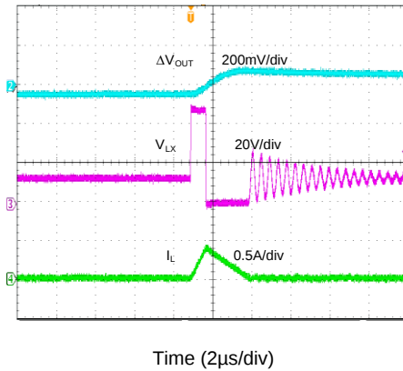
Output Ripple ( V_{\text{IN}}=48\text{V}, V_{\text{OUT}}=12\text{V}, I_{\text{O}}=0\text{A} )
