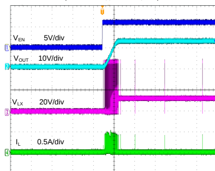
Startup from EN ( V_{IN}=48V , V_{OUT}=12V , I_O=0A )
