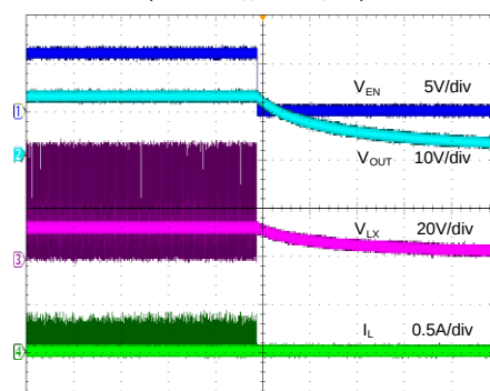
Shutdown from EN ( V_{IN}=48V , V_{OUT}=12V , I_O=0A )
