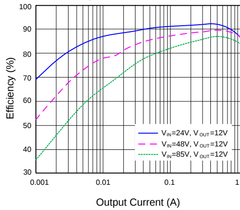
Efficiency vs. Output Current ( L=68\mu\text{H}/\text{CDRH8D43-680NC} )
