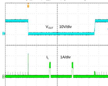
Hard Short Protection ( V_{IN}=48V , V_{OUT}=12V , I_O=0A \sim Short)
